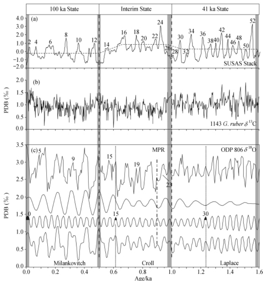
Fig. 6. Subdivision of the last 1.6 Ma of the Quaternary into major climate stages based on the evolution of oceanic carbon system. (a) Triple division into “100 ka State,” “Interim State” and “41 ka State” based on Subtropical South Atlantic Susceptibility (SUSAS) stack [36] ; (b) triple division based on four \delta^{13}\text{C}_{\text{max}} events, represented by planktonic \delta^{13}\text{C} of ODP Site 1143, SCS; (c) triple division into “Milankovitch”, “Croll”, and “Laplace” chrons based on predominant climate cyclicity represented by benthic \delta^{18}\text{O} of ODP 806, western tropical Pacific [24] .
