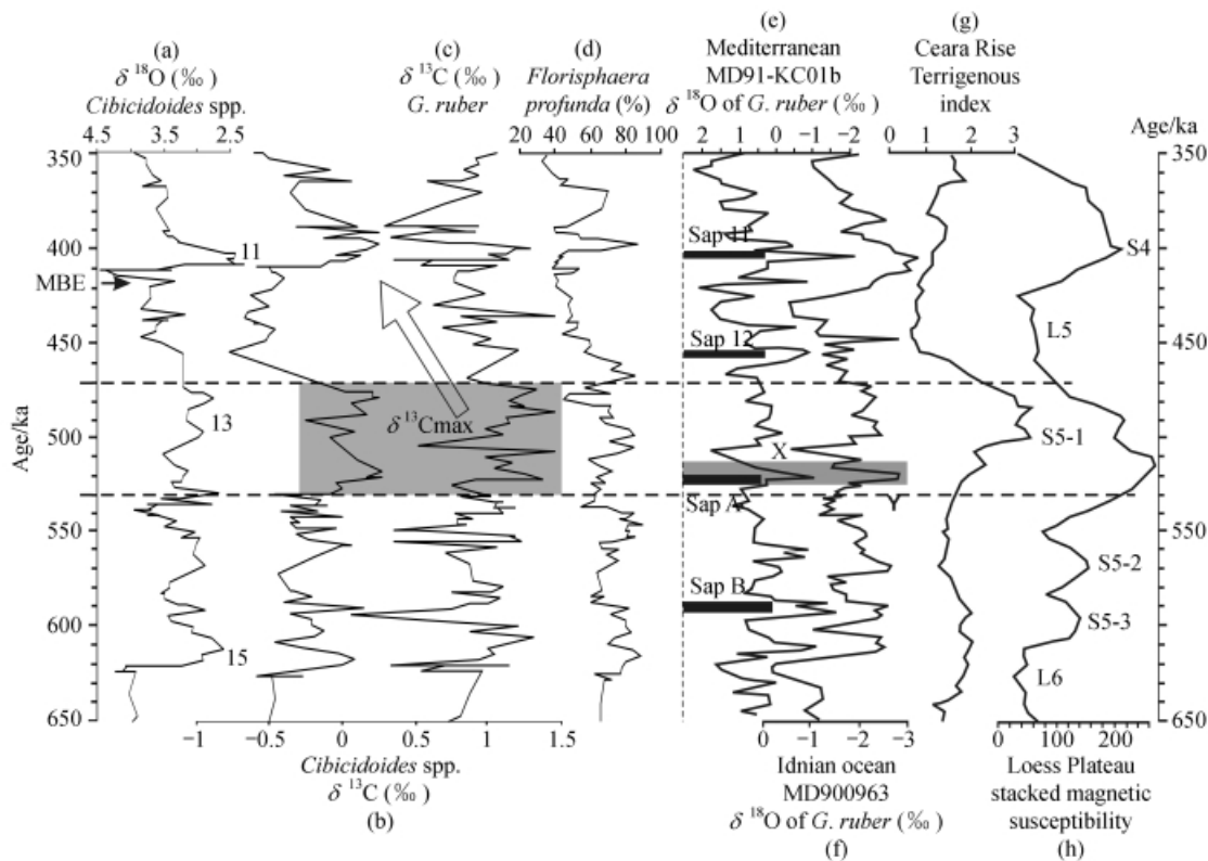
Fig. 4. Records of events around the \delta^{13}\text{C}_{\text{max-II}} in MIS 13. ODP Site 1143, SCS: (a) Benthic \delta^{18}\text{O} (MBE—Mid-Brunhes Event); (b) benthic \delta^{13}\text{C} ; (c) plankton \delta^{13}\text{C} ; (d) nannoplankton Florisphaera profunda %. Other oceans: (e) planktonic \delta^{18}\text{O} record with sapropel layers (Sap) in core KC01b, Mediterranean ( 36^{\circ}15' \text{N} , 17^{\circ}44' \text{E} , w.d. 3643 m): “Sap A” is abnormal [27] ; (f) planktonic \delta^{18}\text{O} record in core MD 900963, equatorial Indian Ocean ( 5^{\circ}03' \text{N} , 73^{\circ}52' \text{E} , w.d. 2446 m), showing \delta^{18}\text{O} events Y and X [26] ; (g) “Terrigenous index” (relative terrigenous mass accumulation rate) at ODP Sites 929/925, equatorial Atlantic [28] ; (h) stacked magnetic susceptibility from Loess Plateau, China (S, paleosol; L, loess) [29] .
