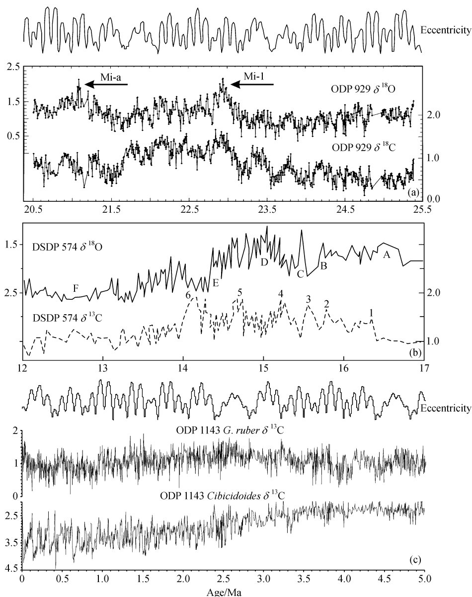
Fig. 7. Comparison of deep-sea benthic \delta^{18}\text{O} and \delta^{13}\text{C} records over three time intervals in the late Cenozoic: (a) Late Oligocene-early Miocene, 20.5–25.4 Ma, ODP Site 929, western equatorial Atlantic ( 5^{\circ}58' \text{N} , 43^{\circ}44' \text{W} , w.d. 4358 m), compared with orbital eccentricity [37] ; (b) Middle Miocene, 12–17 Ma, DSDP Site 574, eastern equatorial Pacific ( 4^{\circ}12' \text{N} , 133^{\circ}19' \text{W} , w.d. 4561 m), A–F denote \delta^{18}\text{O} events, 1–6 denote \delta^{13}\text{C}_{\text{max}} events CM1–CM6 [39] ; (c) Plio-Pleistocene, 0–5 Ma, ODP Site 1143, southern SCS, compared with orbital eccentricity.
