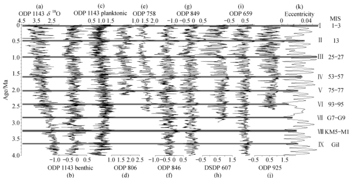
Fig. 2. A global correlation of \delta^{13}\text{C} curves for the last 4 Ma (for locations and water depth see Table 1). Western Pacific: ODP 1143 (a) benthic \delta^{18}\text{O} ; (b) benthic \delta^{13}\text{C} ; (c) planktonic \delta^{13}\text{C} ; (d) ODP 806 planktonic \delta^{13}\text{C} [14] . Indian Ocean: (e) ODP 758 planktonic \delta^{13}\text{C} [18] . Eastern Pacific: (f) ODP 846 benthic \delta^{13}\text{C} [17] ; (g) ODP 849 benthic \delta^{13}\text{C} [16] . Northern Atlantic: (h) DSDP 607 benthic \delta^{13}\text{C} [20] ; (i) ODP 659 benthic \delta^{13}\text{C} [21] ; (j) ODP 925 benthic \delta^{13}\text{C} [22] ; (k) eccentricity. Gray bars denote the carbon isotope maximum events ( \delta^{13}\text{Cmax} ) showing 400–500 ka periodicity, and \delta^{13}\text{Cmax} corresponds to eccentricity minimum (k) before the Quaternary. I—IX on the right show the succession of \delta^{13}\text{Cmax} .
