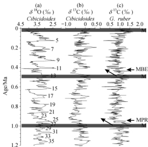
Fig. 3. Oxygen and carbon isotopic records spanning 1.2 Ma from ODP Site 1143. (a) Benthic \delta^{18}\text{O} ; (b) benthic \delta^{13}\text{C} ; (c) planktonic \delta^{13}\text{C} . Numbers labeling \delta^{18}\text{O} curve indicate marine oxygen isotope stages (MIS), grey bars denote carbon isotope maximum ( \delta^{13}\text{C}_{\text{max}} ), MBE stands for Mid-Brunhes Event, MPR for Mid-Pleistocene Revolution. Arrows show that \delta^{13}\text{C}_{\text{max}} preceded the transition in glacial cyclicity and expansion of ice-sheet [13] .
