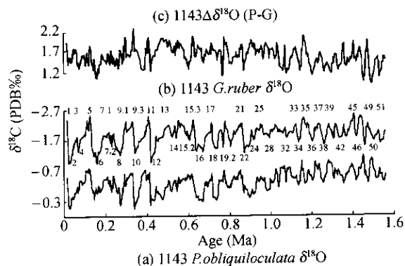
Fig. 2. Comparison of P. obliquiloculata \delta^{18}\text{O} (a), G. ruber \delta^{18}\text{O} (b) and \delta^{18}\text{O}(\text{P-G}) (c) after 5-point running smoothing in the last 1.56 Ma. The numbers denote some Marine Isotope Stages.
