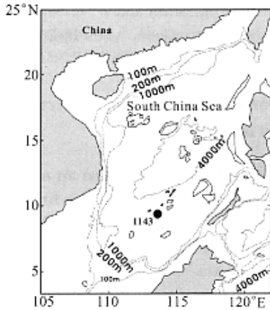
Fig. 1. Location map of ODP Site 1143.
