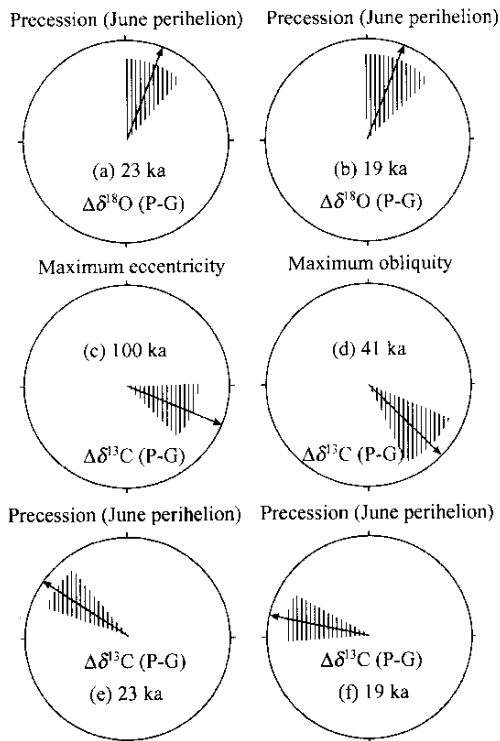
Fig. 5. Phase wheels of the \Delta\delta^{18}\text{O} (P-G) and the \Delta\delta^{13}\text{C} (P-G) relative to the ETP. (a) \Delta\delta^{18}\text{O} (P-G), at the 23-ka band; (b) \Delta\delta^{18}\text{O} (P-G), at the 19-ka band; (c) \Delta\delta^{13}\text{C} (P-G), at the 100-ka band; (d) \Delta\delta^{13}\text{C} (P-G), at the 41-ka band; (e) \Delta\delta^{13}\text{C} (P-G), at the 23-ka band; (f) \Delta\delta^{13}\text{C} (P-G), at the 19-ka band. The phase values are from Table 1.
