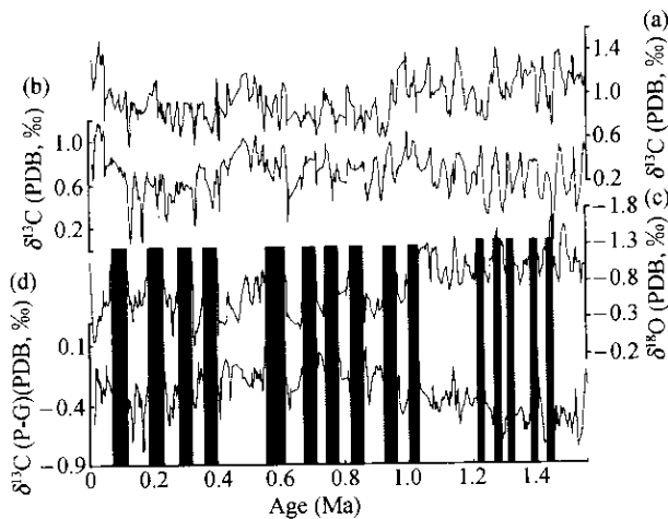
Fig. 3. Comparison of G. ruber \delta^{13}\text{C} (a), P. obliquiloculata \delta^{13}\text{C} (b), P. obliquiloculata \delta^{18}\text{O} (c) and \Delta\delta^{13}\text{C}(\text{P-G}) (d) after 5-point running smoothing in the last 1.56 Ma. Shaded bars denote interglacials. Numbers denote some Marine Isotope Stages.
